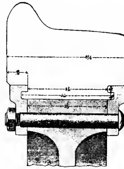
Fig. 5339. THE MANSELL TIRE FASTENING Fastenings for Steel-tired Wheels in General Use.
